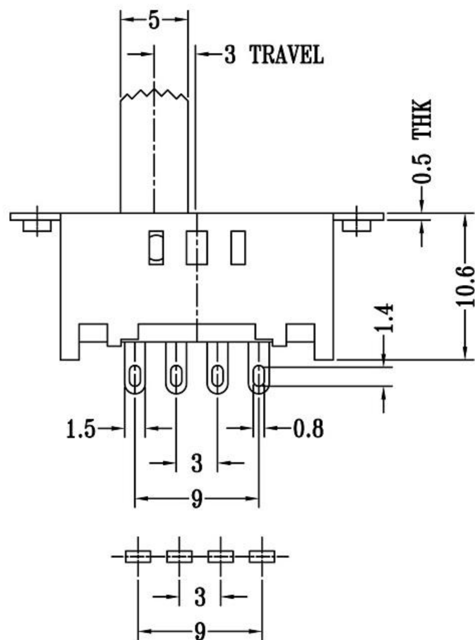
P.C.B LAYOUT BOTTOM VIEW
